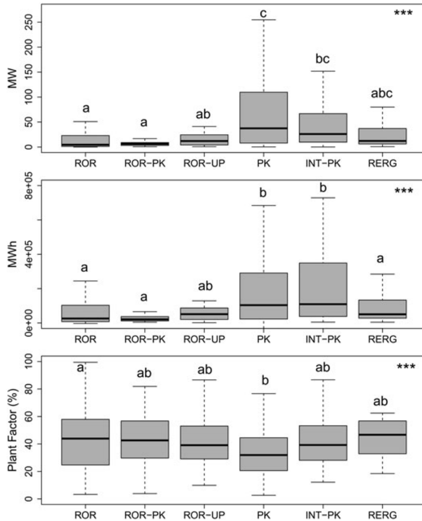
Figure 5. Box and whisker plots of characteristics for power plants according to modes of operation (MOPs). *, **, and *** represent statistical significant among MOPs at the 0.05, 0.005, and 0.0001 levels using Kruskal–Wallis tests. Different letters represent statistical significance of non-parametric pair-wise comparisons at the p < 0.05 level
