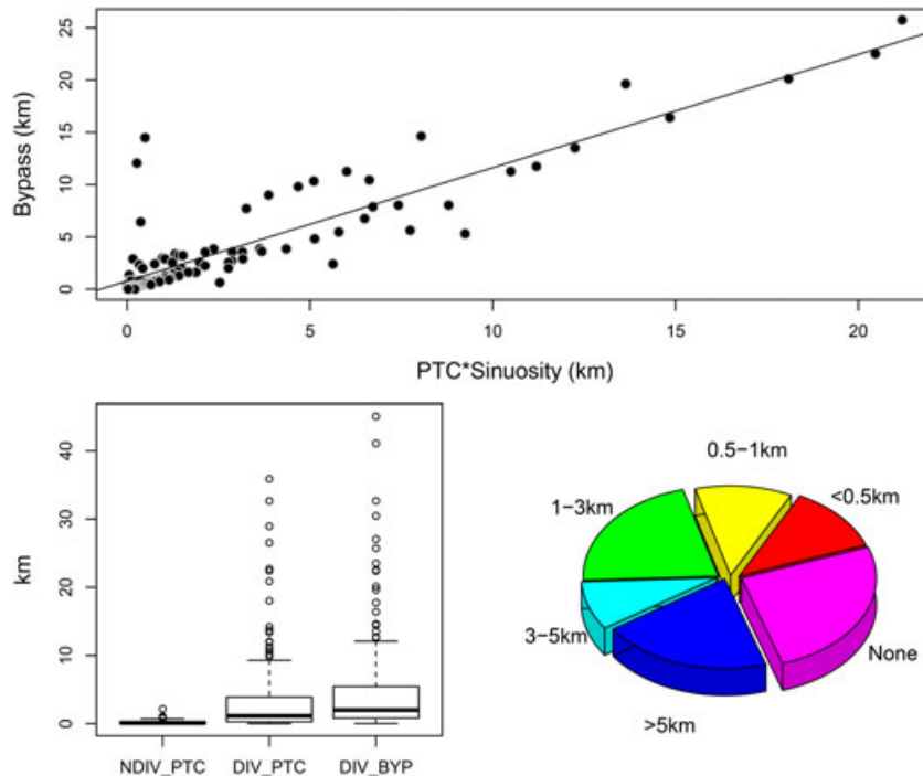
Figure 2. Analysis of diversion-bypass at hydropower dams ( n = 284 ) regulated by the Federal Energy Regulatory Commission. (A) Summed values of lengths for penstock, tunnels, and canals (PTC) were multiplied by channel sinuosity and compared to empirical values of bypass ( n = 103 ) using linear regression. (B) Lengths were compared among PTCs for non-diversion scenarios, PTCs for diversion scenarios, and diversion-bypass lengths. (C) The distribution of bypass lengths among diversion scenarios were examined only for FERC hydropower dams. 'None' indicates that length values were not provided for PTCs or bypasses in FERC documents. This figure is available in colour online at wileyonlinelibrary.com/journal/tra
