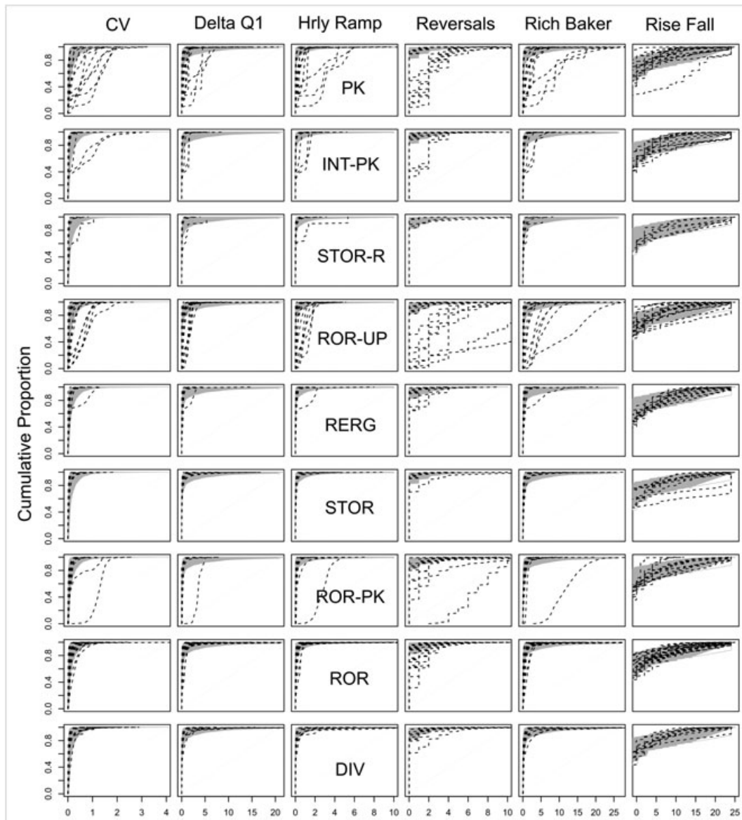
Figure 9. Cumulative frequency distribution (CFD) plots of six sub-daily hydrologic indices (columns) and nine modes of operation (rows). Each line represents a separate CFD for an individual stream gauge over four years. Grey shaded region represents the maximum and minimum of the 95 th percentile values for 35 reference streams across the US
