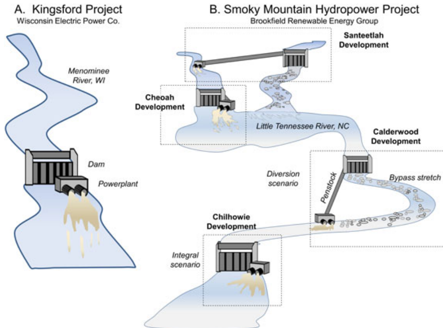
Figure 1. Conceptual model of different hydropower scenarios depicting (A) an integral dam and powerhouse and (B) a complex project consisting of multiple developments and a combination of integral and non-integral (i.e. diversion) dam/powerplant configurations. This figure is available in colour online at wileyonlinelibrary.com/journal/rra
