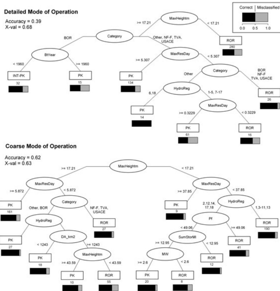
Figure 8. Classification trees predicted detailed modes of operation (MOPs) and coarse MOPs for powerplants. Numbers below each node represent sample sizes. Accuracy refers to % of samples accurately classified. X-val refers to cross-validation error rate
