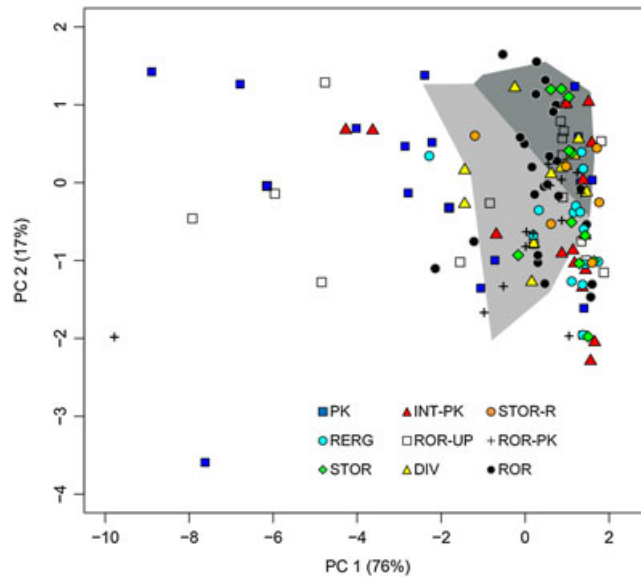
Figure 10. Ordination of stream gages regulated by different dam operations using Principal Components Analysis (PCA) on six subdaily flow metrics. Dark polygon outlines the smallest multidimensional space occupied by 90% of the reference streams. Lighter polygon outlines the entire multidimensional space occupied by all reference streams. This figure is available in colour online at wileyonlinelibrary.com/journal/rra
