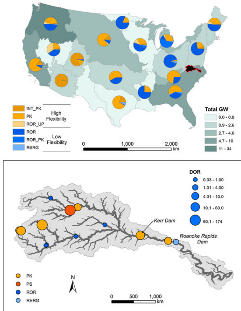
Figure 11. Flexibility in hydropower dam operations across the conterminous US (top). Pie charts represent proportion of gigawatt (GW) capacity represented by each mode of operation. Hydropower dams in the Roanoke River Basin according to operation and degree of regulation (DOR). This figure is available in colour online at wileyonlinelibrary.com/journal/rra
