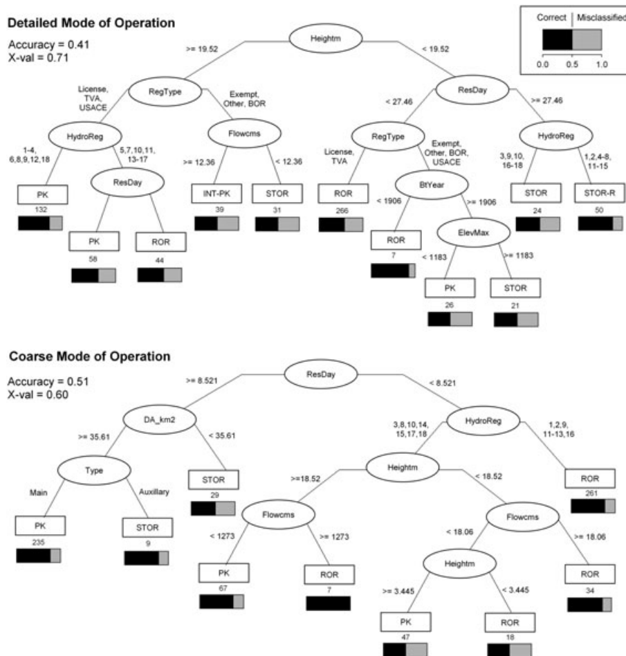
Figure 7. Classification trees predicted detailed modes of operation (MOPs) and coarse MOPs for dams. Numbers below each node represent sample sizes. Accuracy refers to % of samples accurately classified. X-val refers to cross-validation error rate
